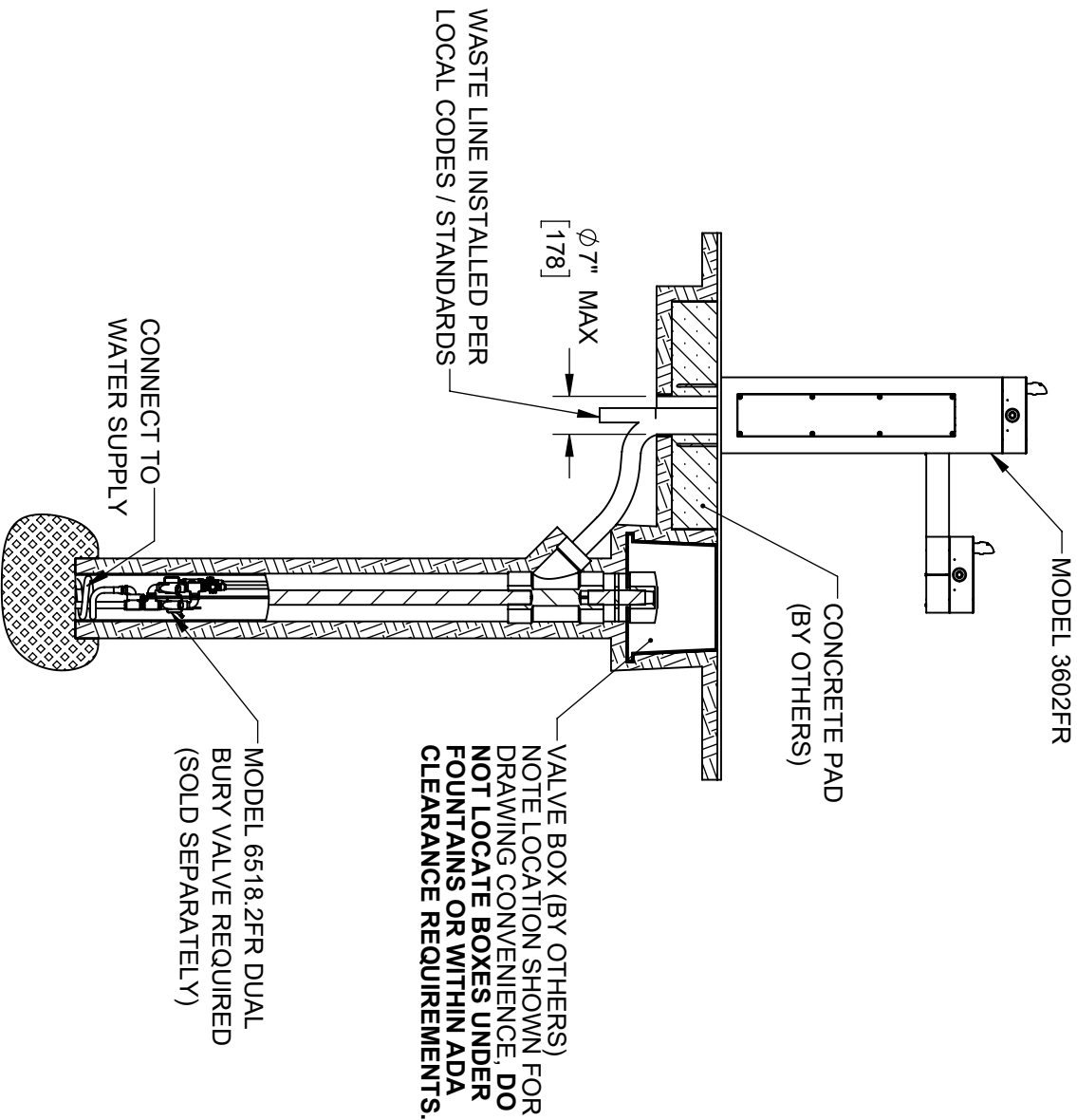
3602FR GENERAL BURY VALVE LAYOUT (FOR REFERENCE ONLY)
