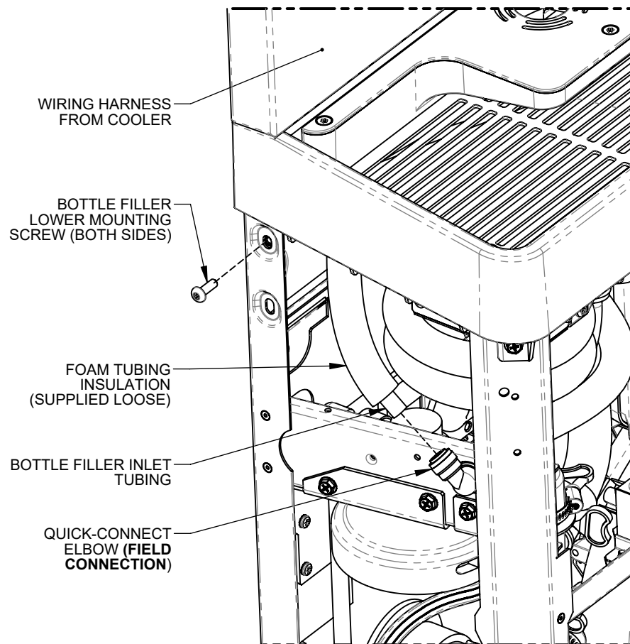
BOTTLE FILLER MOUNTING & TUBING CONNECTION
