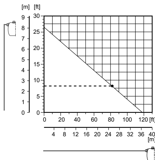
Maximum inlet-pipe length (horizontal axis) according to the suction lift (vertical axis)
