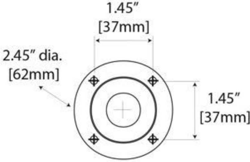
Wall Flange Detail
