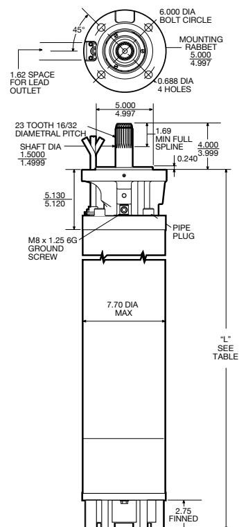
Type 1.0 (40-150 hp)
