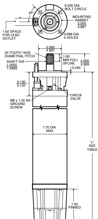
Type 2.1 (40-100 hp)
