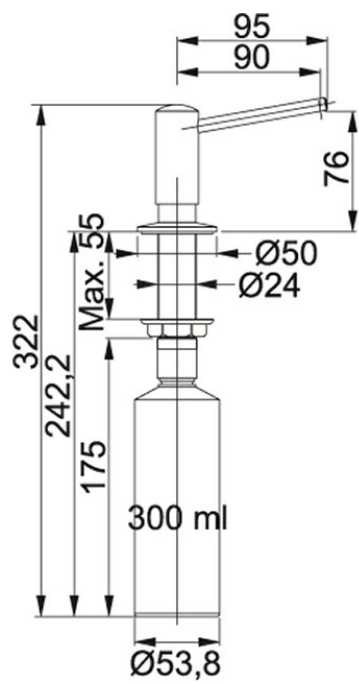
Technical Drawing
