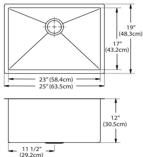
Dimensional Drawing
