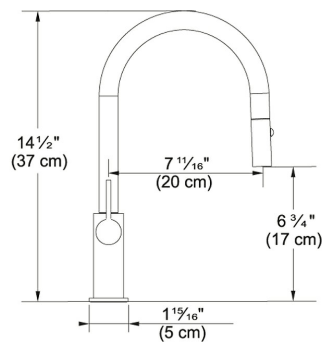
Technical Drawing
