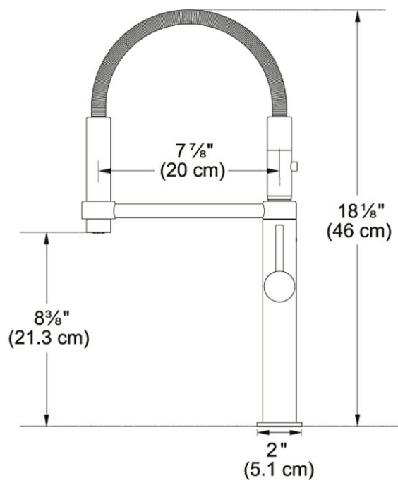
Technical Drawing
