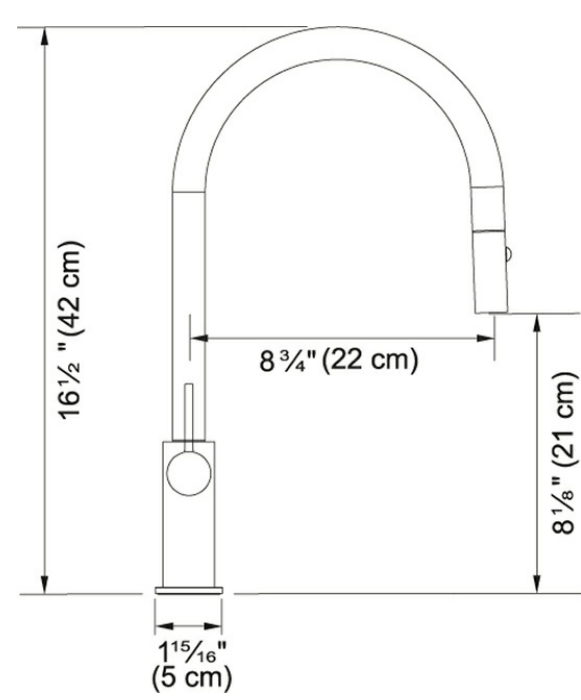
Technical Drawing
