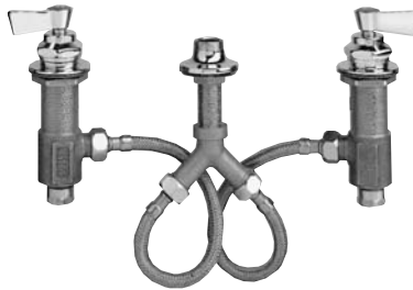
#2232 — Widespread Deck Control Valve w/ swivel outlet #2658 — Widespread Deck Control Valve w/ swivel outlet, check valve #2259 — Widespread Deck Control Valve w/ 3/8"F outlet #2666 — Widespread Deck Control Valve w/ 3/8"F outlet, check valve
