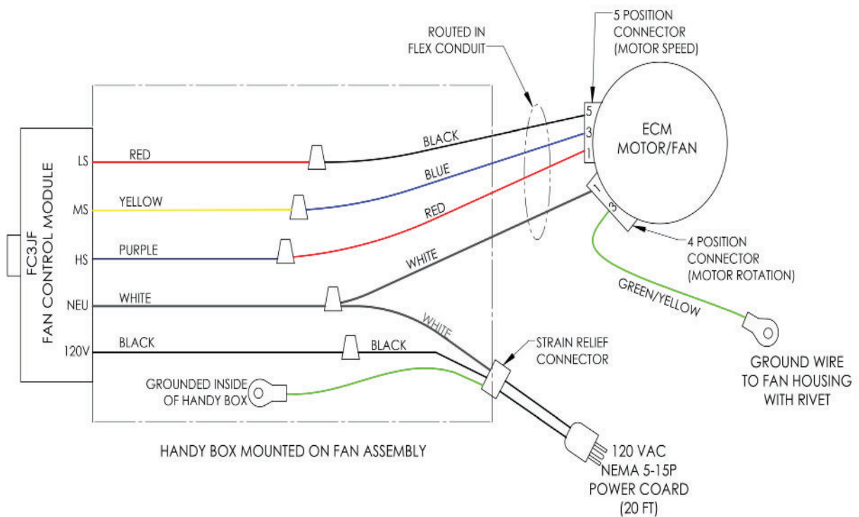
DIAGRAM 2: VC SUMMIT S2-S6.5 (GEN4) FAN WIRING
