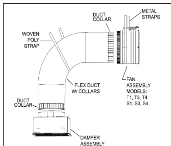
FIGURE 3A: FLEX DUCT TO FAN ASSEMBLY CONNECTION (MODELS: S3 and S4)
