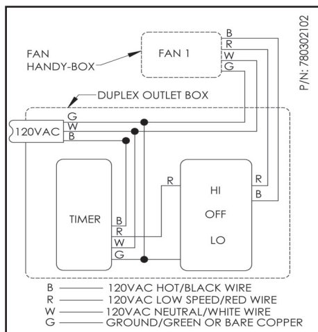
ELECTRICAL - 2 SPEED CONTROL (HARDWIRED)
