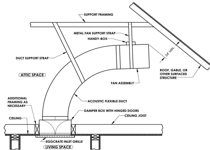
TYPICAL INSTALLATION - VENTCOOL TAHOE SERIES
