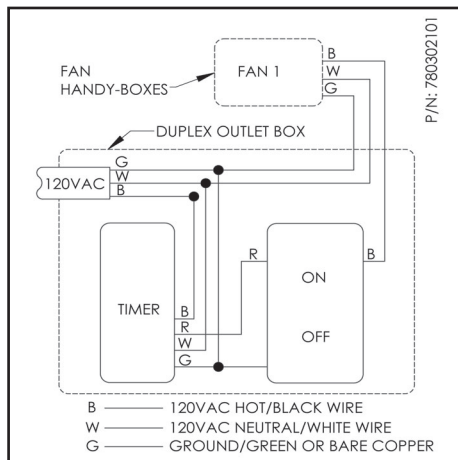
ELECTRICAL - SINGLE SPEED CONTROL (HARDWIRED)
