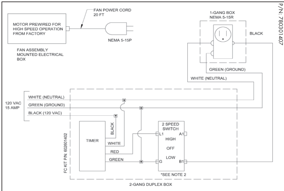
DIAGRAM 1: For T2-T5 Models with 2 Speed Control Switch using Fan Power Cord
