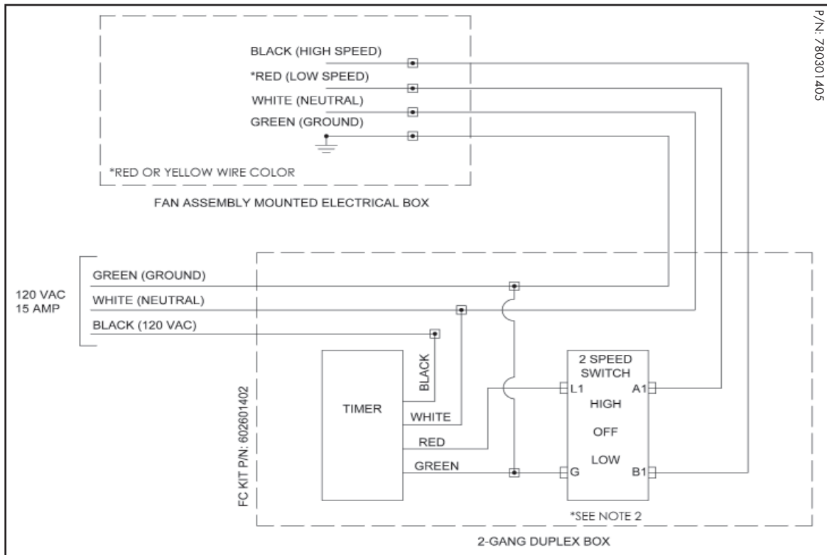
DIAGRAM 2: For T2-T5 Models with 2 Speed Control Switch Hardwired to Fan Assembly
