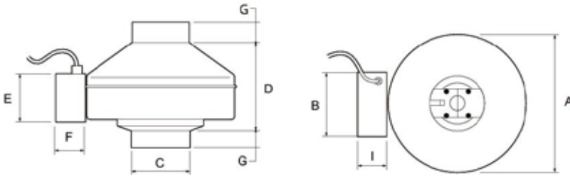
Dimensions (inches)
