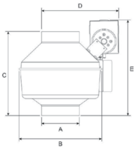
Dimensions (inches)
