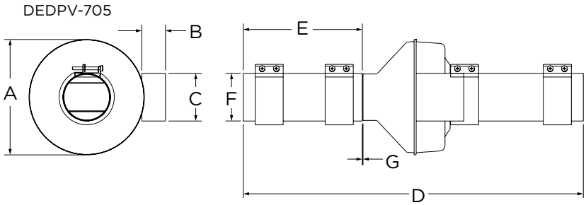
Dimensions (inches)
