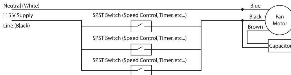
Multiple Location Switching Wiring Diagram
