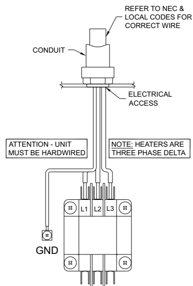
WIRING CONNECTION
