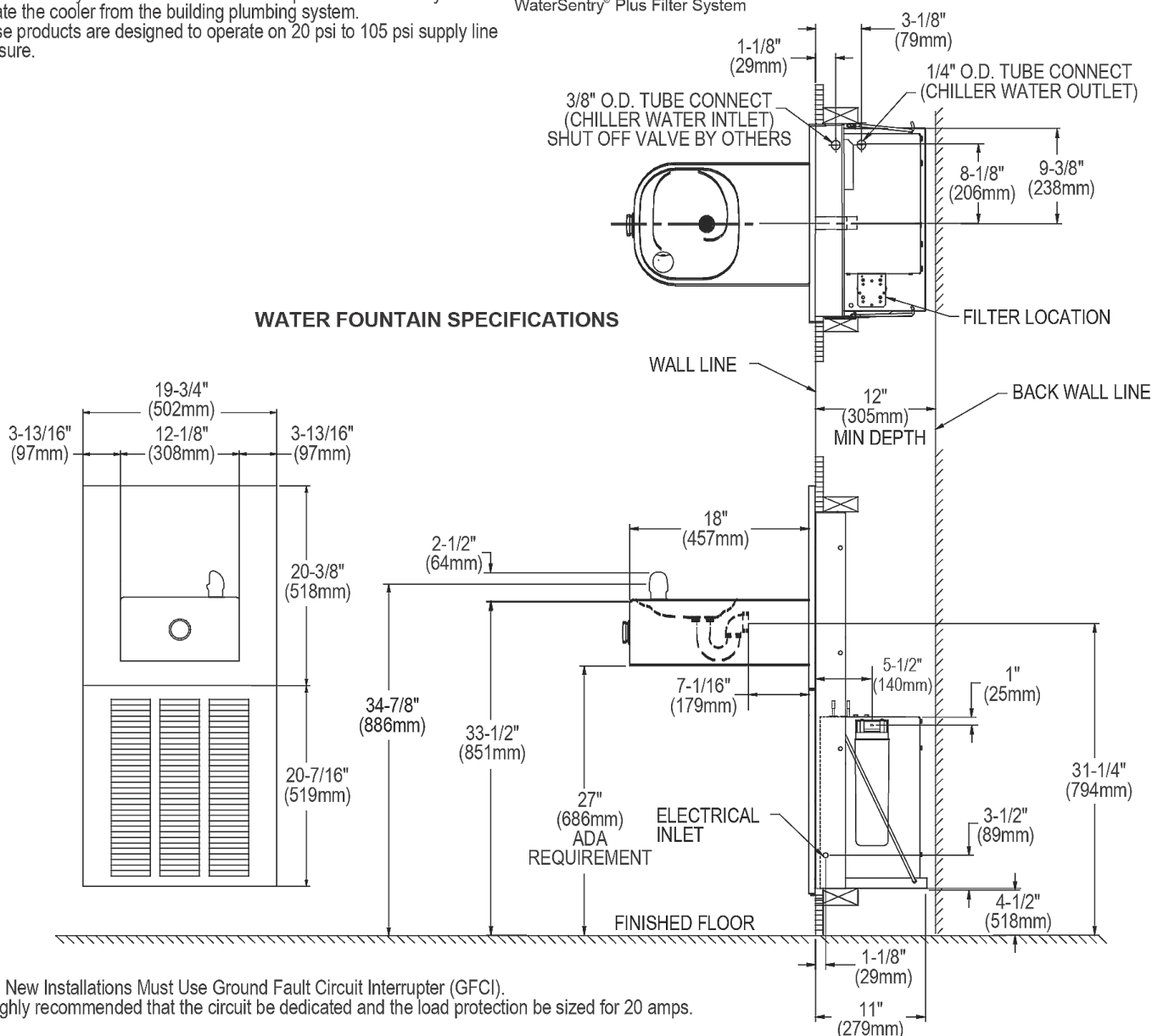
WaterSentry® Plus Filter System
