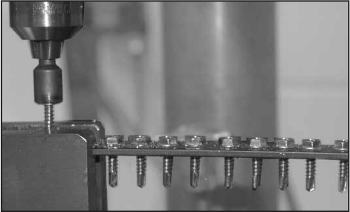
DRILL POINT LENGTH MUST EXCEED TOTAL THICKNESS
