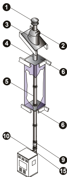
Multi-Story FasNSeal
