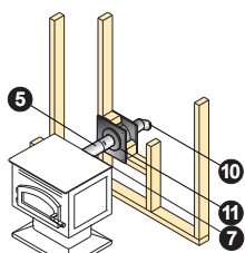
Through-The-Wall
