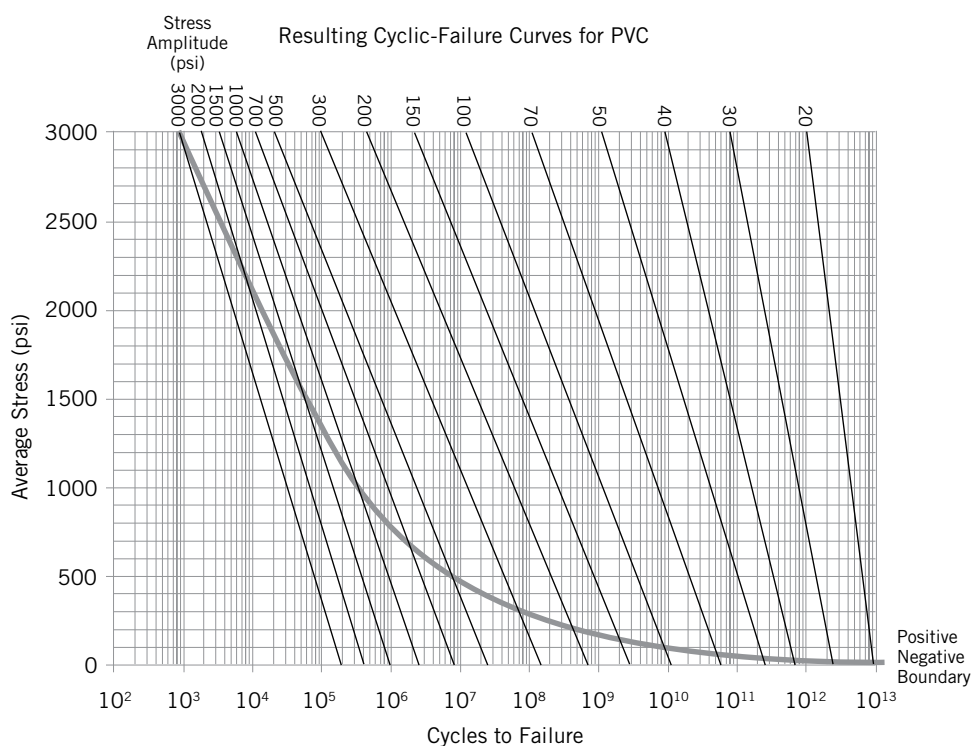
Figure 3 – Resulting Cyclic-Failure Curves for PVC
