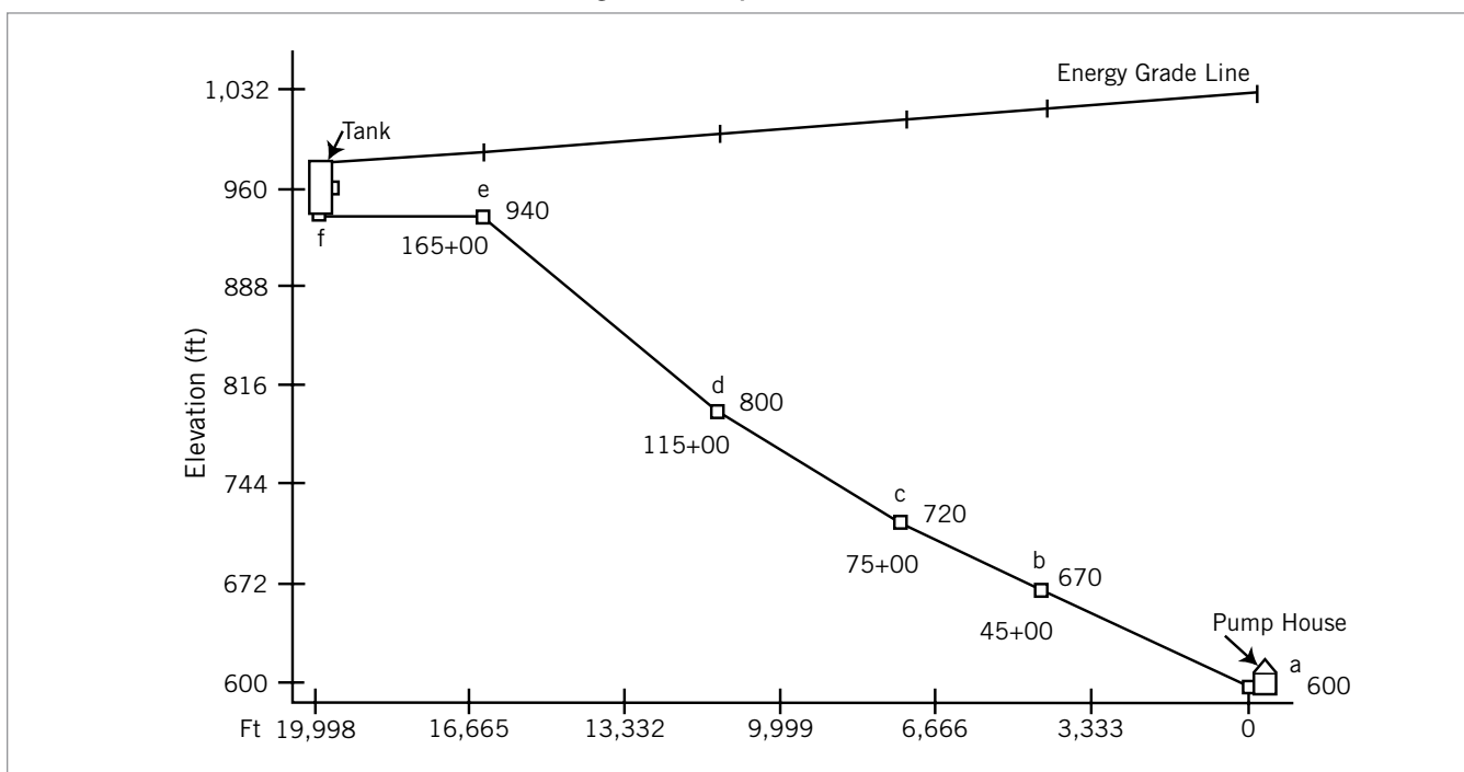
Figure 4 – Pipeline Profile
