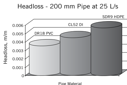
Figure 2 – Pipe Material
