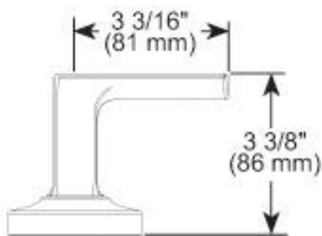
HL70406-▲ Lever Handle
