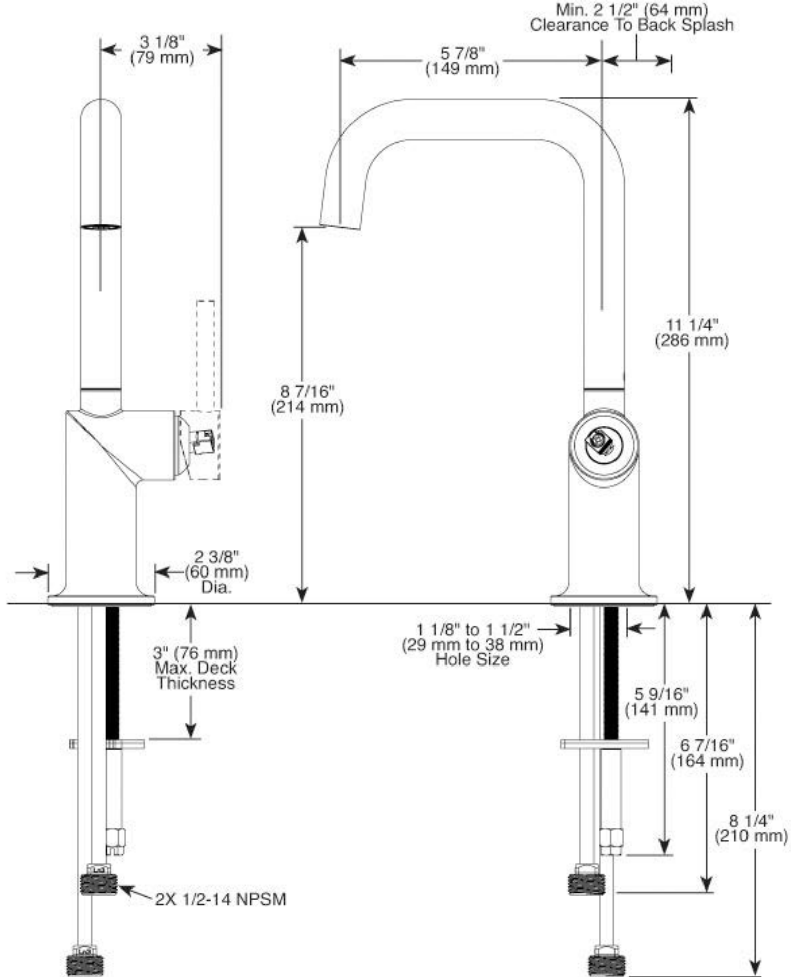
HLB175-▲ Lever Handle
