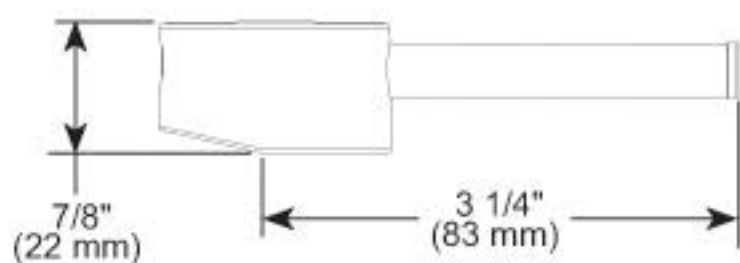
HLB177-▲ Lever Handle
