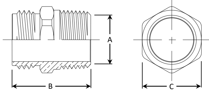
HU22-8-12 & HU22-12-12 - Male Hose Thread x MIP
