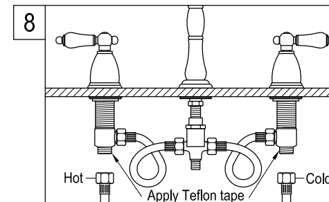
Teflon Tape
