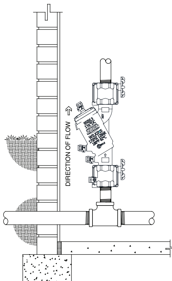
VERTICAL INSTALLATION
