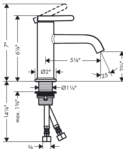
Scale drawing
