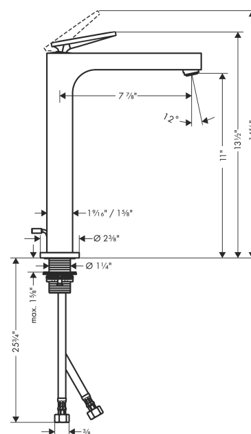
Scale drawing
