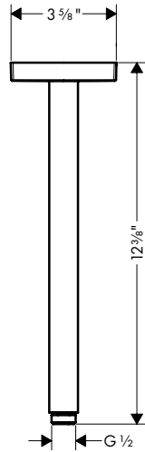
AXOR 300 Ceiling Showerarm Square / SoftSquare 26438XX1 / 26966XX1
