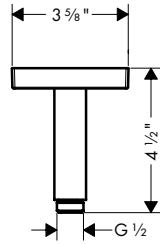
AXOR 300 Ceiling Showerarm Square / SoftSquare 26438XX1 / 26966XX1
