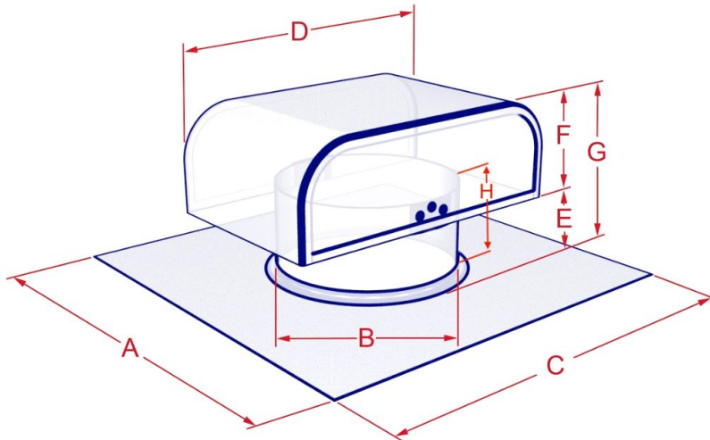
3 PIECE HOOD STYLE SIZES: 5", 7", 8"-12"
