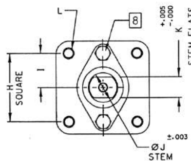
ACTUATOR MOUNTING
