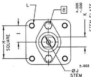
ACTUATOR MOUNTING
