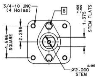
ACTUATOR MOUNTING: 8"
