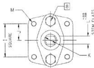
ACTUATOR MOUNTING
