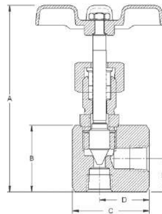
ANGLED VALVE
