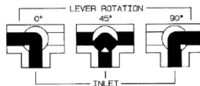
FLOW PATTERN
