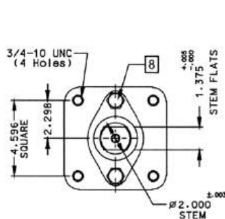
ACTUATOR MOUNTING: 8"
