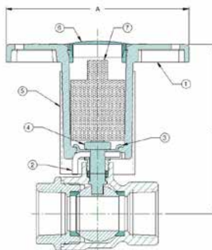
Figure 2: Sectional View
