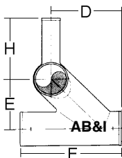
FIGURE 8 DOUBLE EXTENDED WITH FULL BAFFLE
