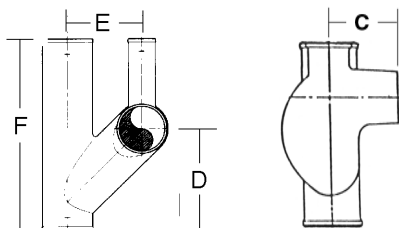
FIGURE 6 DOUBLE EXTENDED with FULL BAFFLE
