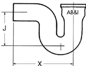
DEEP SEAL "P" TRAP
