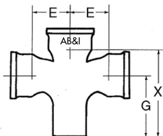
SAN CROSS (No Baffle)
