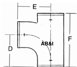
SANITARY TEE
