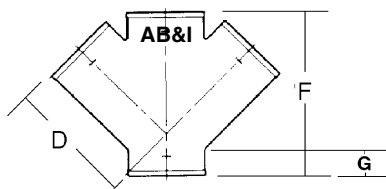
DOUBLE WYE (45°)
