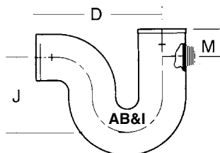
"P" TRAP (with 1/2" Tap Primer)
