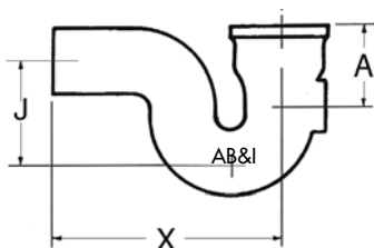
"P" TRAP w/1/2" HEEL TAP
